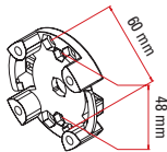
Support standard (6 trous vis M5) max 20 Nm
